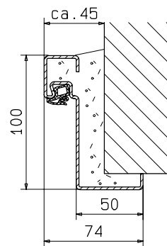
Hauptzarge "ZG 68/76"
